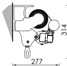
Stenska mont. z ekstrudiranim nosilcem Wall installation with extruded bracket
