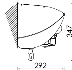
Montaža s strehico Installation with a hood
