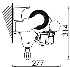
Stenska mont. z ekstrudiranim nosilcem Wall installation with extruded bracket
