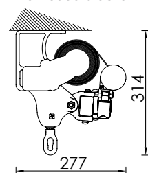
Stropna mont. z ekstrudiranim nosilcem Ceiling installation with extruded bracket
