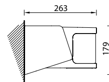
Stenska montaža Wall installation
