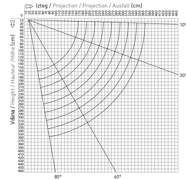
Stenska montaža Wall installation
